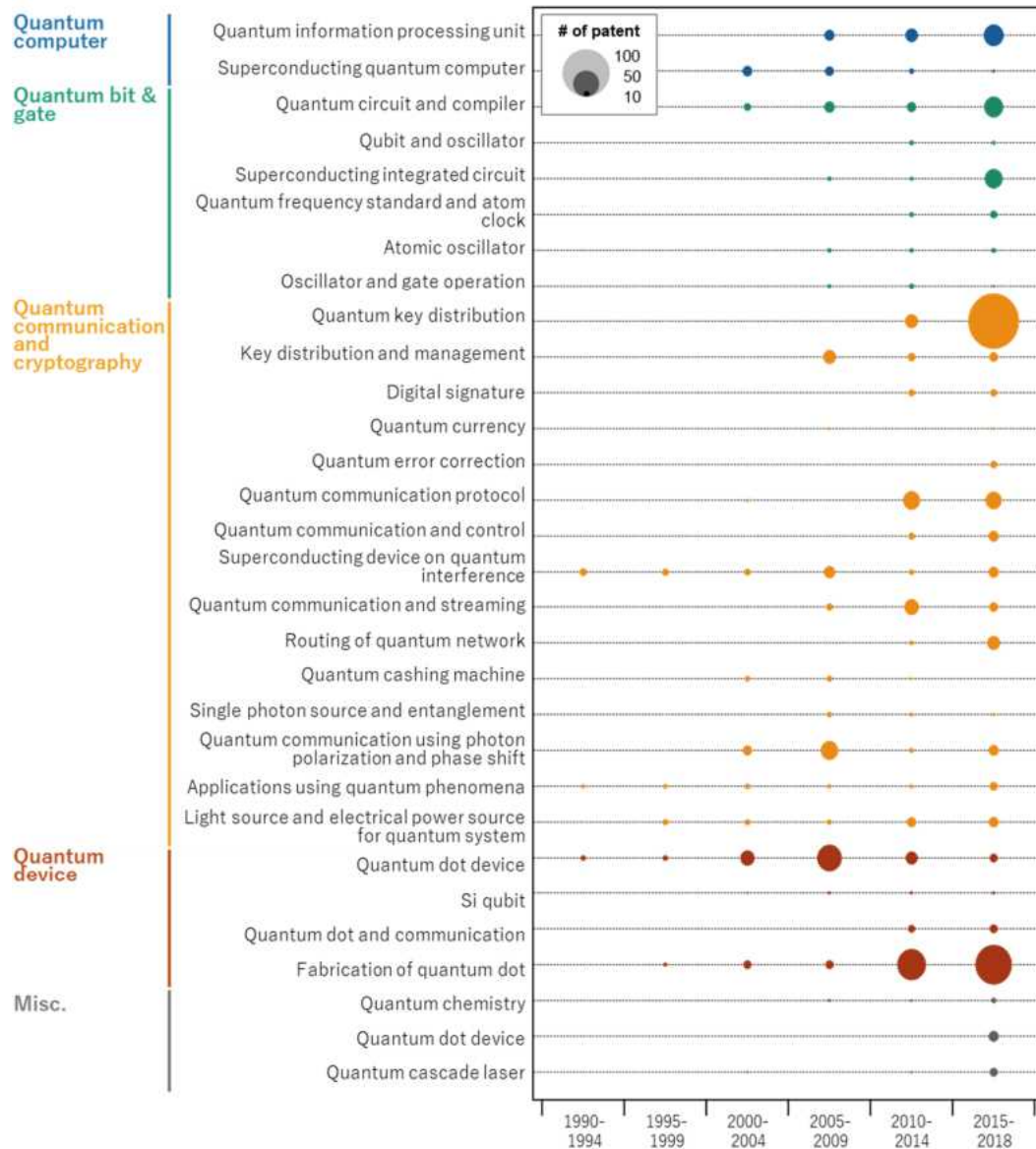
Fig. 6 Trends in the number of patents related to quantum technology [12]
