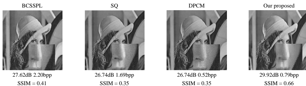
Figure 2. Comparison of visual qualities and compression artifacts of four test images: Lenna, Goldhill, Mandrill, and Pentagon among our proposal, BCSSPL, SQ, and DPCM with B = 4 ,
