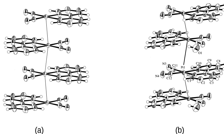
図 2. [\text{Pt}(\text{CN})_2(\text{bpy})] のスタッキング構造: (a) Red Form, \text{Pt} \cdots \text{Pt} = 3.3385(1) \text{ \AA} , \text{Pt} \cdots \text{Pt} \cdots \text{Pt} = 168.59(4)^\circ , (b) Yellow Form, \text{Pt} \cdots \text{Pt} = 3.3279(3) \text{ \AA} , 4.6814(3) \text{ \AA} , \text{Pt} \cdots \text{Pt} \cdots \text{Pt} = 132.89(1)^\circ .
