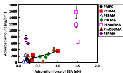
Fig. 10 Relationship between adsorbed amount of protein and adsorption force of BSA at different polymer brush surfaces.
