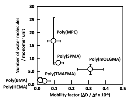
Fig. 11 Mobility factor (Mf) of grafted polymer chains and amount of captured water into polymer brush layers at different polymer brush surfaces.
