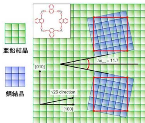
図3-4 亜鉛結晶 [\text{Zn}_2(\text{ndc})_2(\text{dabco})] と銅結晶 [\text{Cu}_2(\text{ndc})_2(\text{dabco})] の構造相関図。
