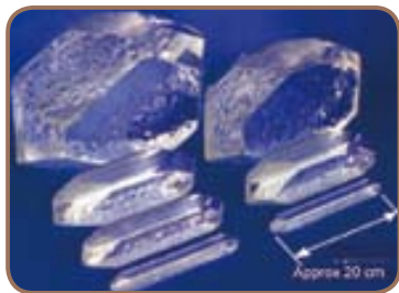
Artificial crystal
