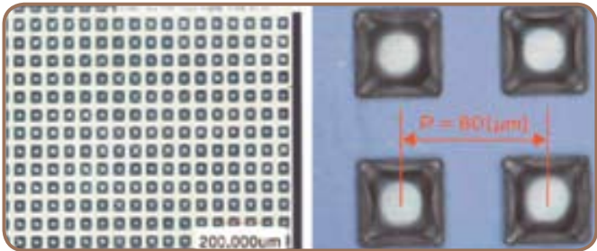
80 \mu\text{m} pitch bumps forming photo
