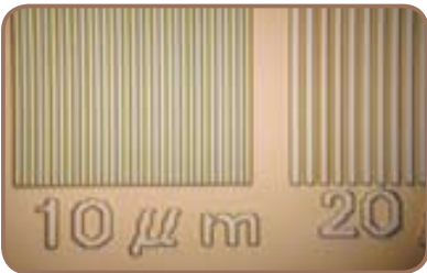
Exposure sample: Liquid resist
