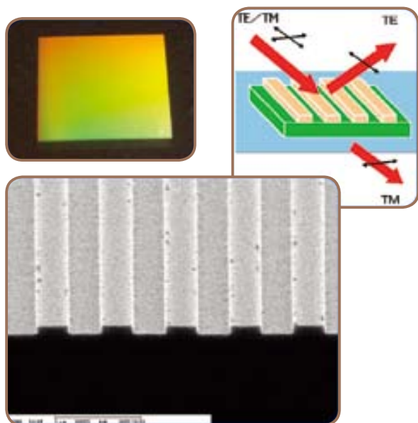
Polarizing splitting element
