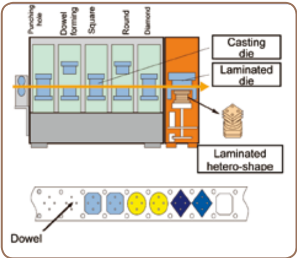
Hetero-shaped lamination method based on this technology
