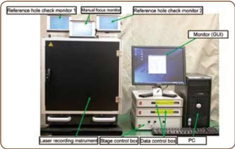
Direct multi-polygon laser instrument: Sample configuration
