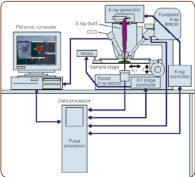
Key diagram of X-ray analytical microscope
