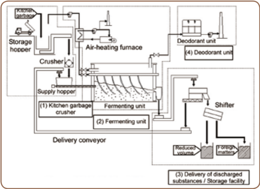
System configuration
