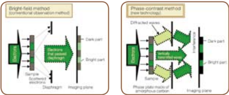
Difference between bright-field method and phase-contrast method
