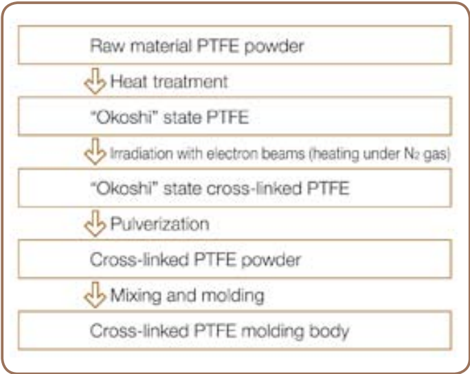
Manufacturing process of cross-linked PTFE
