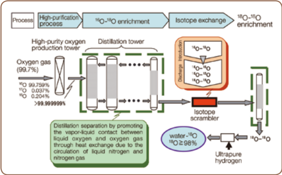
Manufacturing process of water- 18 O distilling
