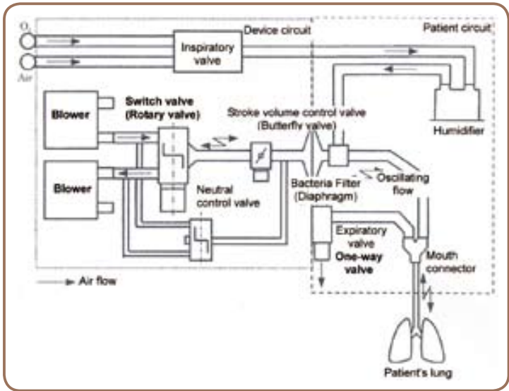
Overview of high-frequency ventilator for adults
