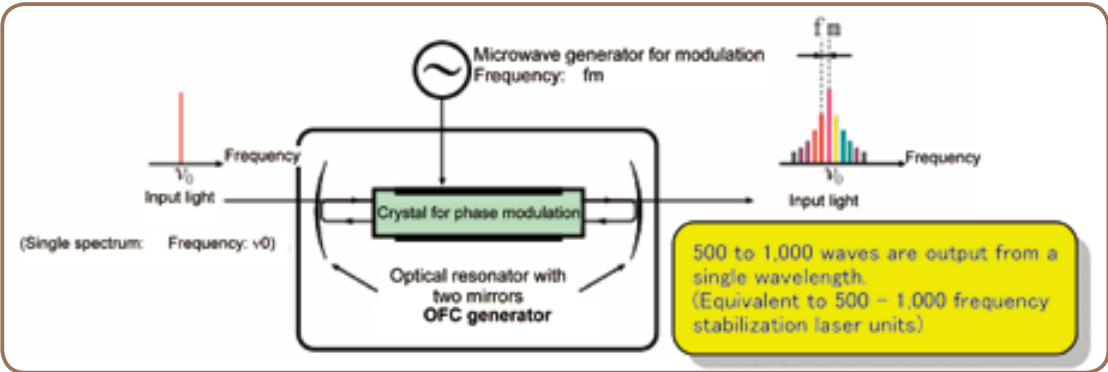
Principle diagram
