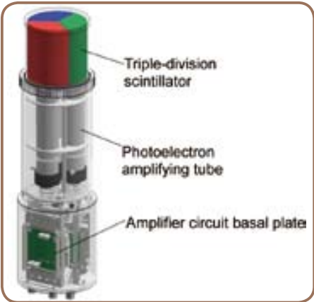
Conceptual view
