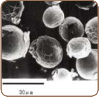
SEM photograph of hollow TiO 2 spheres
