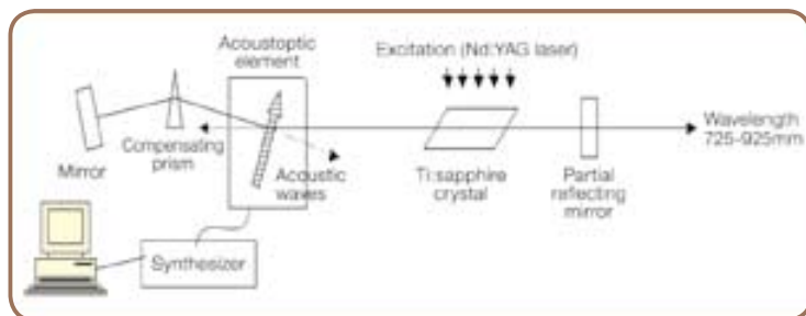
Basic composition
