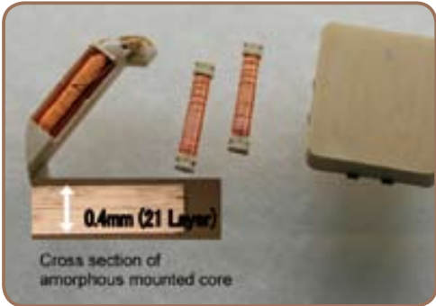
Amorphous antenna
