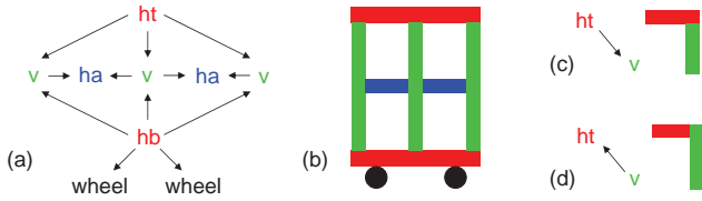
Figure 3: (a) A graph from our example grammar, and (b) the corresponding cabinet. Each node contains the dimensions of each part ( dim_t ). Each edge contains \delta_{a_c} and ( type_c, number_c, transformations_c ). (c,d) The direction of the edges specifies the positioning of the parts. The positionings are important for ensuring that the parts are structurally buildable.
