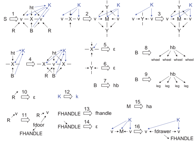
Figure 2: Production rules for 3D cabinets. \epsilon is the empty graph. K represents the back part (blue color is for easier visualization). R is a sub-component for front doors. M is a sub-component for horizontal-adjustable parts and front drawers.
