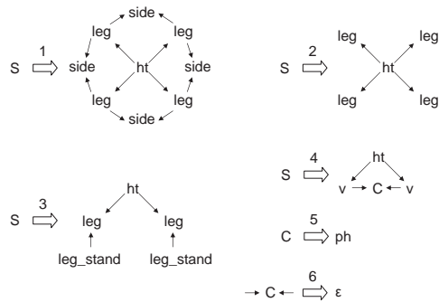
Figure 4: Production rules for 3D tables. ph is an abbreviation for pole-horizontal.
