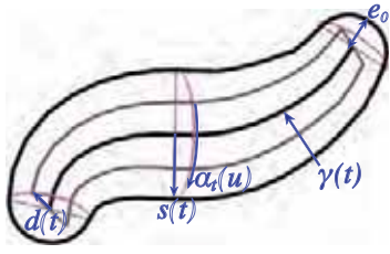
Figure 19: Notation introduced in Section 5.1.
