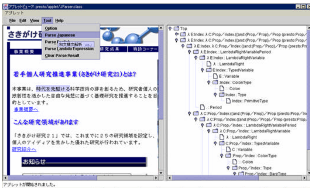
Figure 4: TDL-Parser (JAVA 版)
