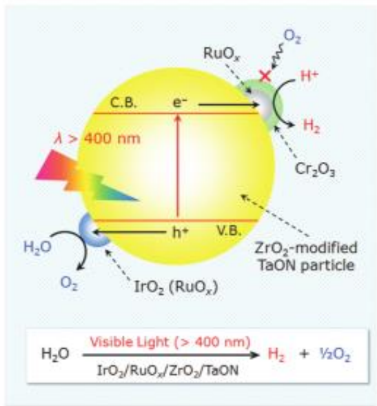
ZrO 2 /TaON光触媒表面を独自のナノ構造化技術で最適化し、反応を高効率化 RuO x (core) Cr 2 O 3 (shell) ナノ粒子 Chem. Eur. J. 2013, 19, 4986–4991. Selected as a Very Important Paper (VIP) and a Frontispiece!
