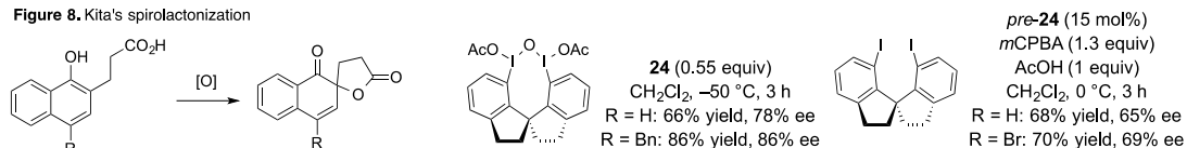
Figure 8. Kita's spiroactonization
