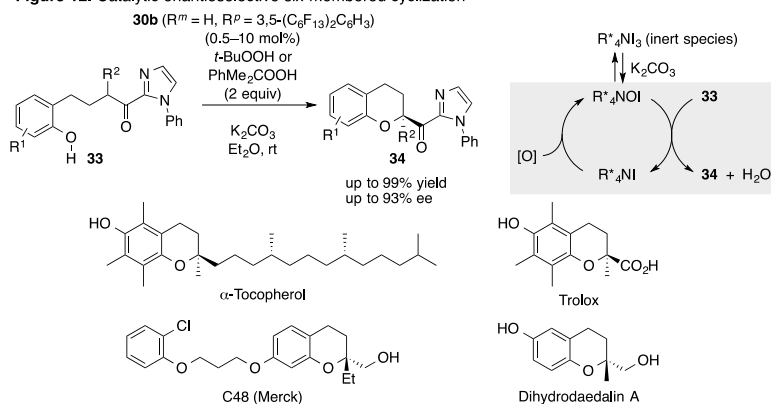
Figure 12. Catalytic enantioselective six-membered cyclization
