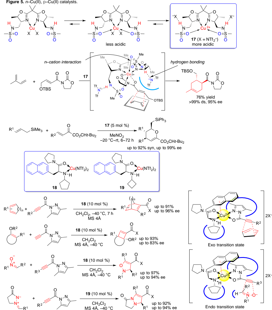
Figure 5. n -Cu(II), \pi -Cu(II) catalysts.
