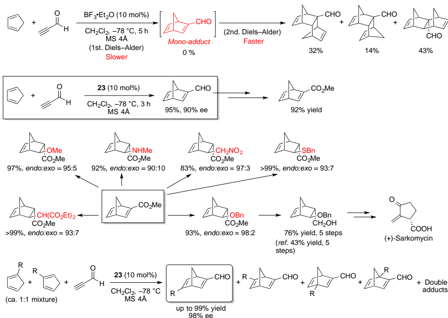
Figure 7. Site-, substrate-, enantio-, and diastereoselective Diels–Alder reaction.
