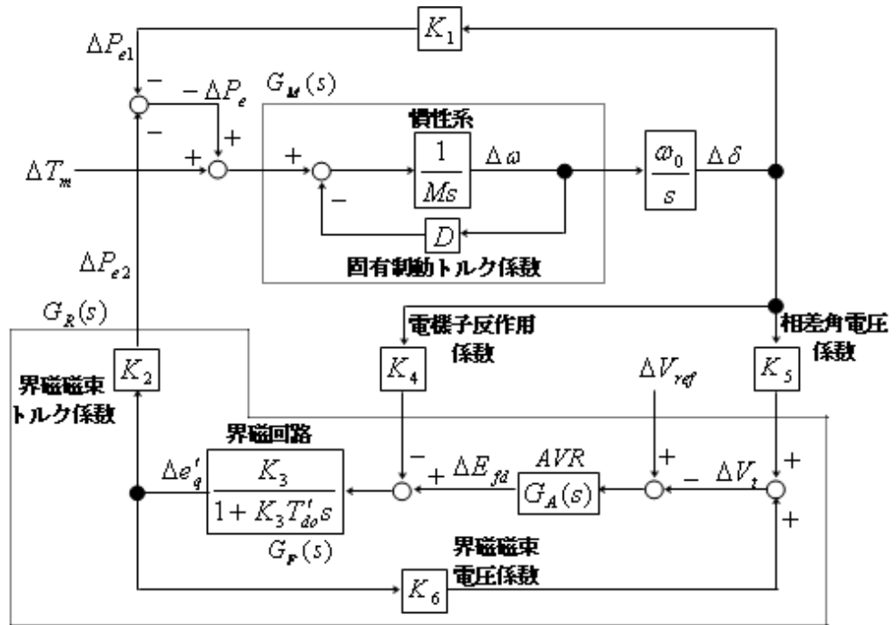
Block diagram of Single Machine Infinite Bus
