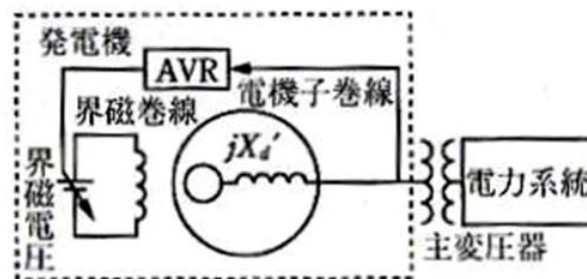
Single Machine Infinite Bus (一機対無限大母線系統)
