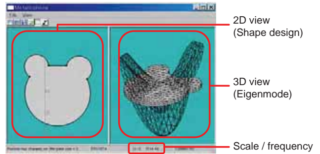
Figure 2: Metallophone design software. The left window is used for the original 2D design, whereas the right window shows the analyzed eigenmode as a 3D graphic. The tone is updated in real time with both audio and visual feedback for the user.
