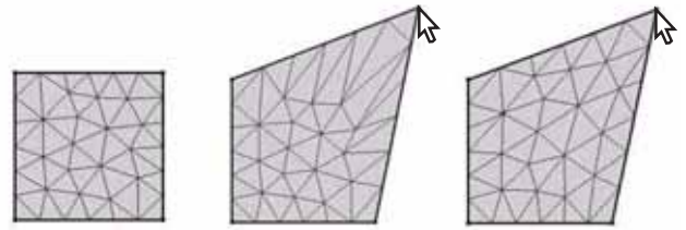
Figure 7: The smoothing of mesh using Laplacian smoothing
